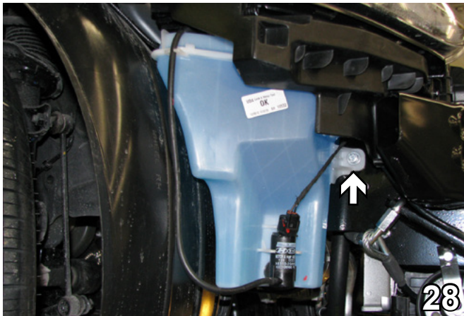
28. Reinstall the washer reservoir with a 6MM-1 x 30MM hex bolt, 1/4" lock washer and 1/4" flat washer into the existing hole on the baseplate. Use the existing bolts previously removed to tighten the other side. Reconnect the hoses.
