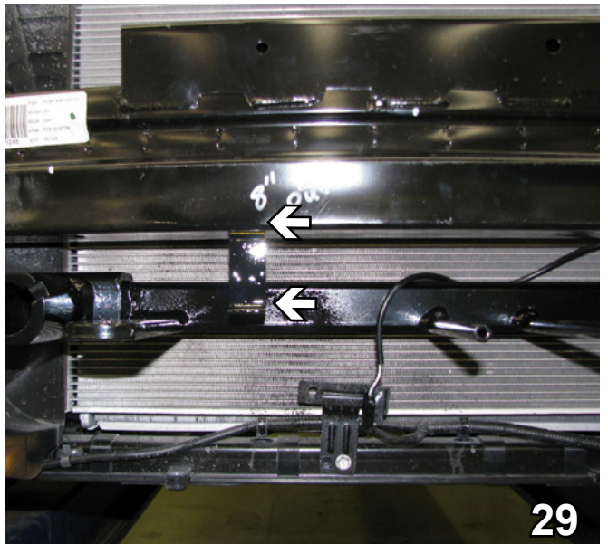
29. Using a 13/32" drill bit, drill through the existing hole in the bottom of the bumper. Attach the breakaway bracket with a 1/4"-20 x 2-1/2" hex bolt and 1/4"-20 hex nut. Attach the breakaway to the bracket with 1/4"-20 x 3/4" hex bolt and 1/4"-20 hex nut.
