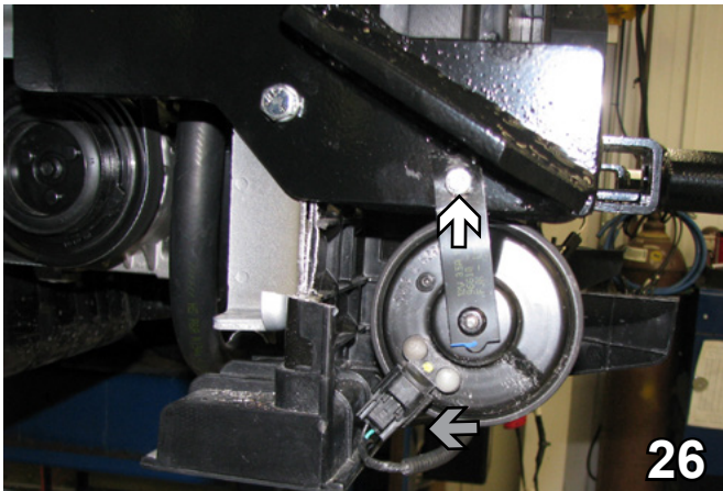
26. On the passenger side, mount the horn on the bottom hole with a 1/4"-20 x 3/4" hex bolt to a 1/4"-20 hex nut (white arrow). Reconnect the plug (gray arrow).
