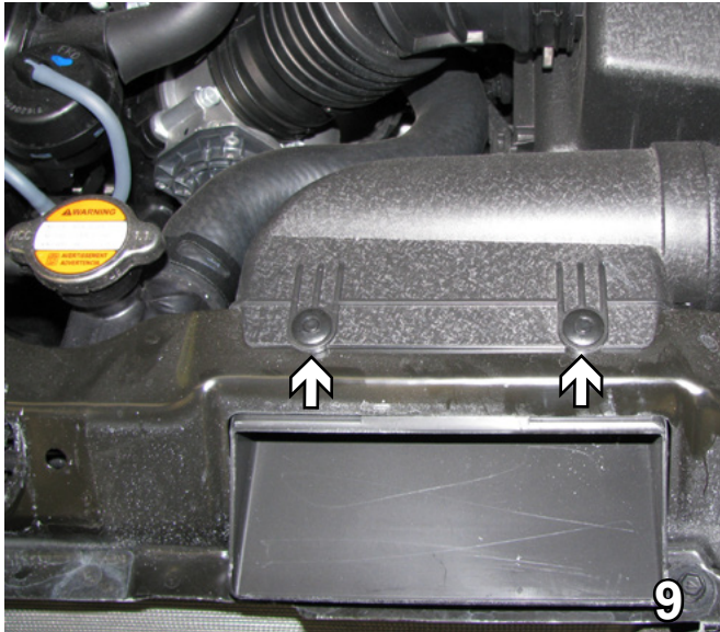
9. On the top front of the car, remove the two (2) push pins before the air baffle can be removed. Push in on each push pin and it will release and pop out.
